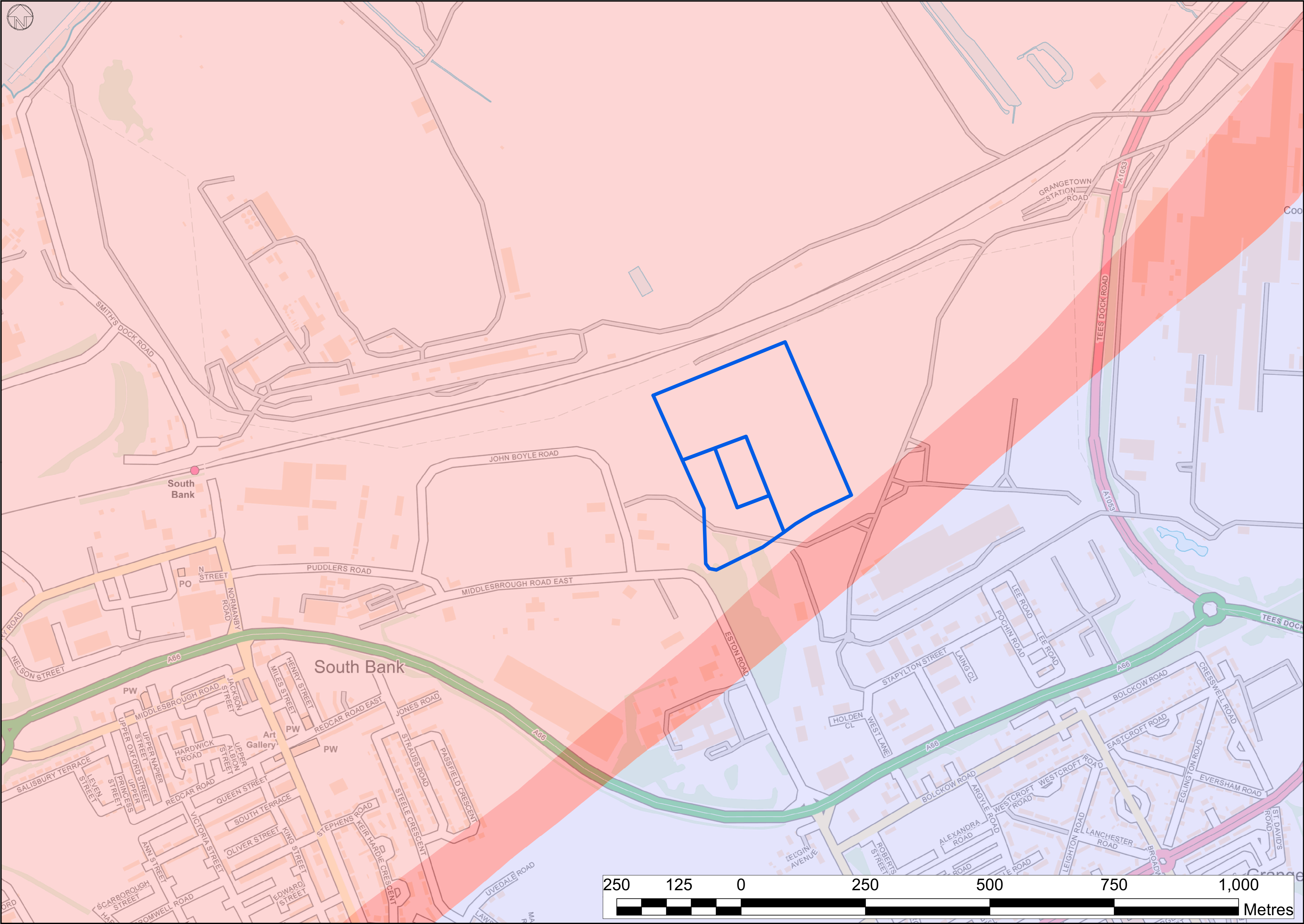
FIGURE 8-4: SOLID GEOLOGY 1:4,000 @ A1 / 1:8,000 @ A3
