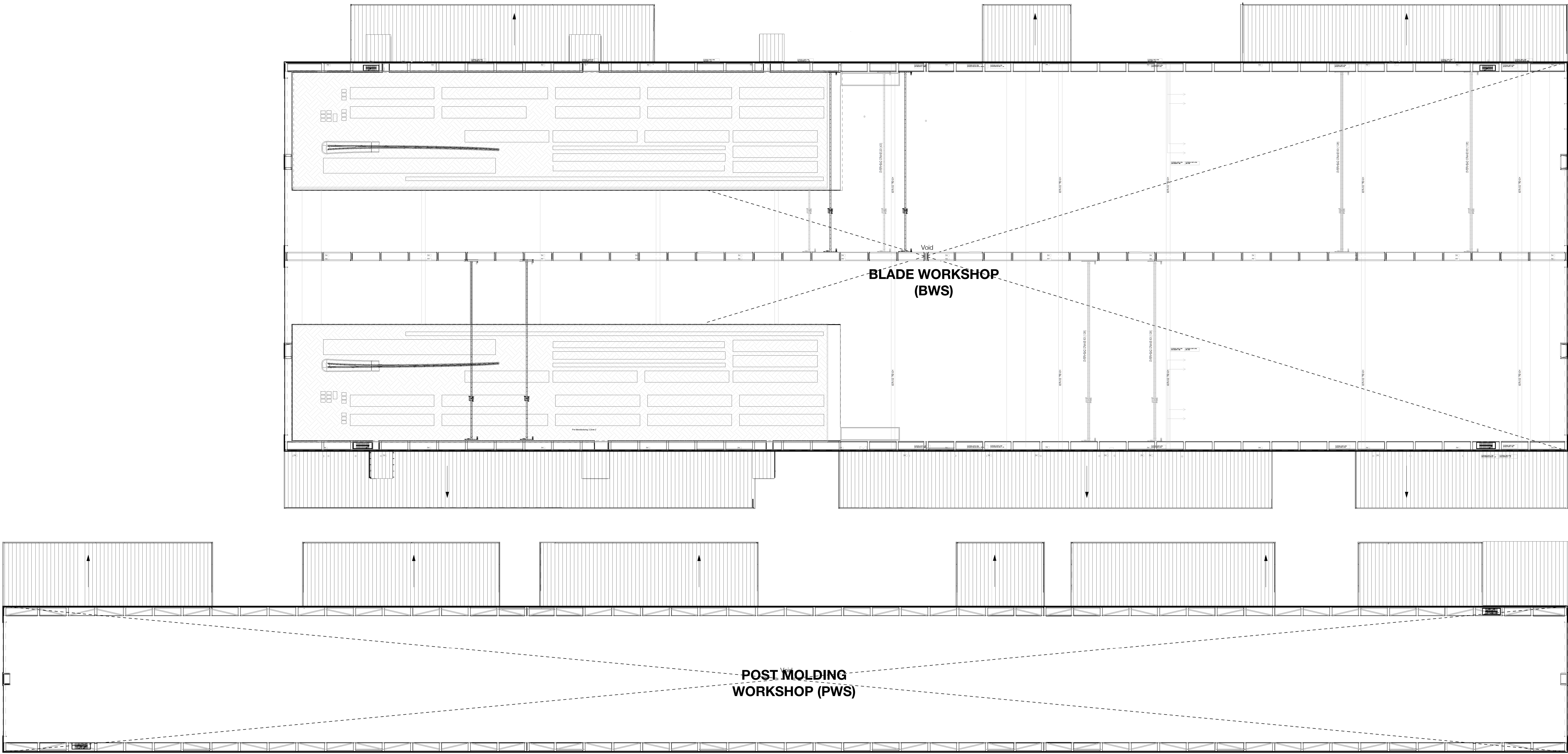
Blade Workshop, Post Molding Workshop & Warehouse GA Plan - Mezzanine 1:600
