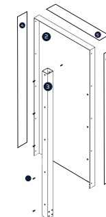
Back Tray
