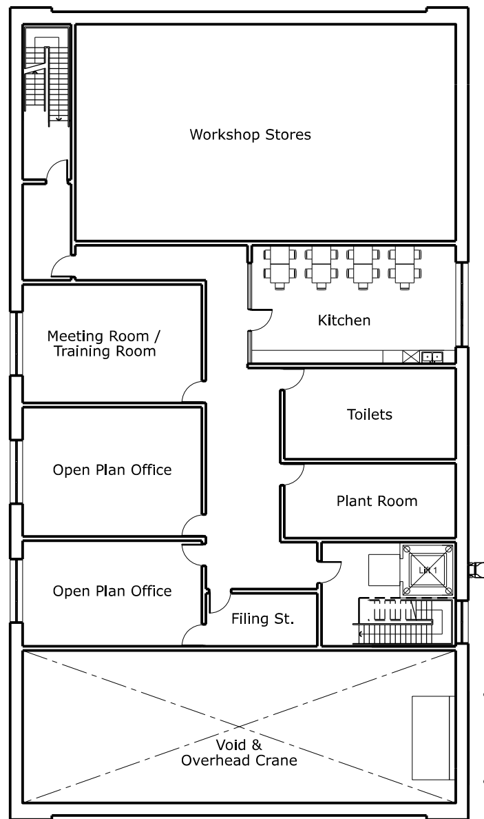
Mezzanine Plan
